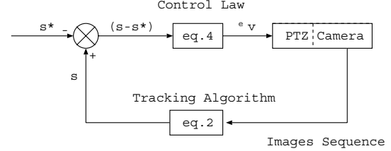
Fig. 7. PTZ Control Synopsis
