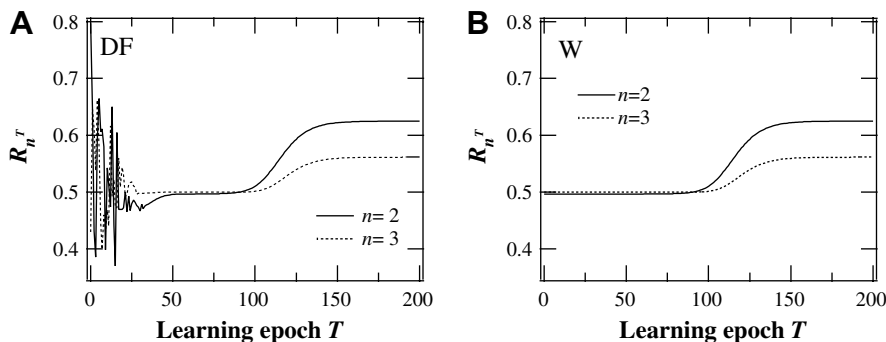
Fig. 3. Evolution of the weighted-fraction of positive feedback loops R_n^{(T)} for loops in DF (A) and \mathcal{W} (B) and circuit length n=2 (thick line) and n=3 (dotted line). The weighted-fraction of positive feedback loops is computed according to R_n^{(T)} = \frac{\sigma_n^{+(T)}}{|\sigma_n^{+(T)}| + |\sigma_n^{-}(T)|} where \sigma_n^{+(T)} (resp. \sigma_n^{-}(T) ) is the sum of the weights of every positive (resp. negative) feedback loops of length n in the network at learning epoch T . The loops are taken either in DF (A) or in \mathcal{W} (B). Values are averages over 20 different networks using \lambda = 0.90 . Standard deviations are omitted for readability purpose. See text for definitions. All other parameters as in Fig. 2.
