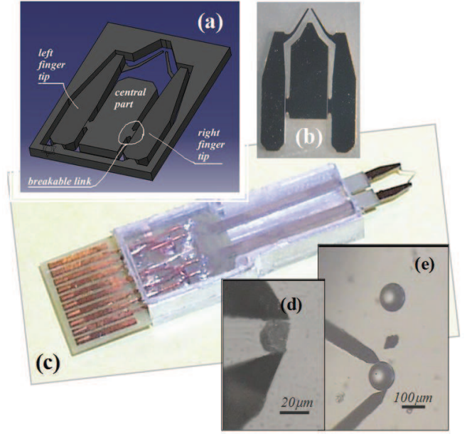
Fig. 1. FEMTO-STs microgripper. (a) and (b): end effectors mounted on breakable parts for easier mounting. (c): MMOC gripper, (d) and (e): handling of micron-sized objects.
