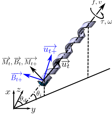
Fig. 1: Magnetic helical swimmer steering model. The inclination angle and direction angle of steering are respectively \theta_i and \theta_d .
