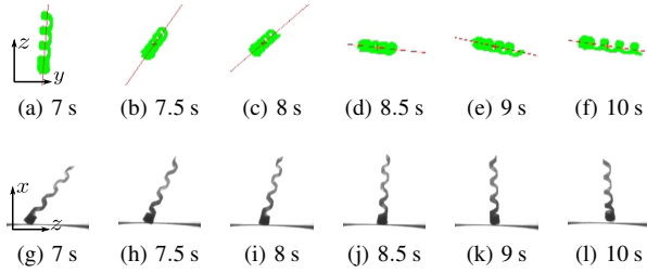
Fig. 6: Images sequence of 90° angle direction steering with 45° inclination angle. (a)-(f) show the top view of the helical swimmer, and (g)-(l) show the side view.
