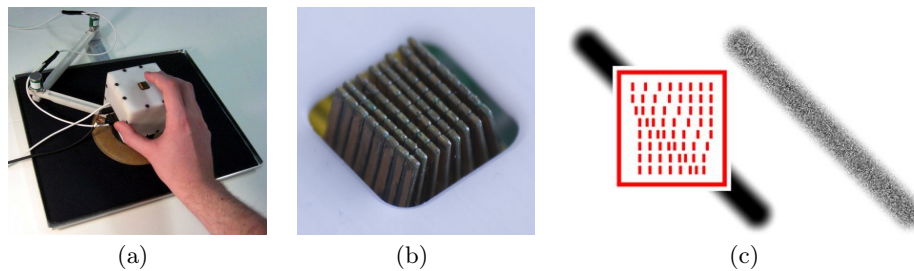
Fig. 1. Pictures of (a) the Tactograph and (b) its array of skin contactors, and (c) simulation of actuator activation over 5-mm wide stroked lines.
